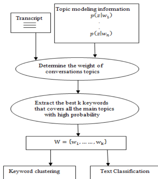
Fig. 1 Keyword based Document Classification
